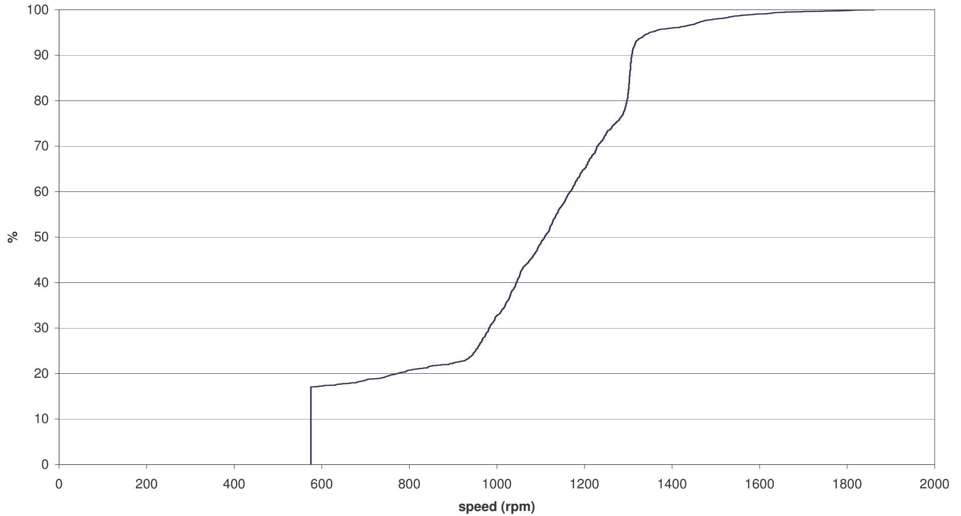
WHTC Speed vs Cumulative Frequency - Example 16 litre engine
