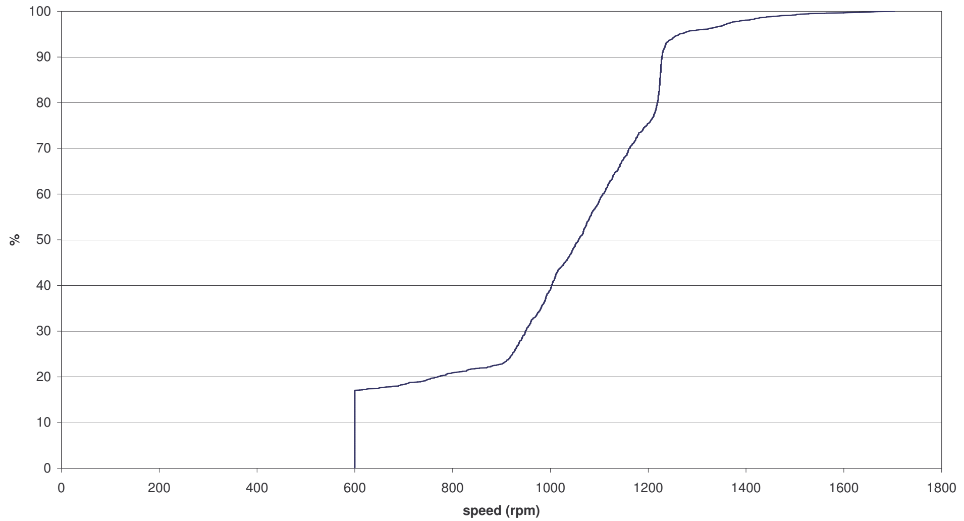
WHTC Speed vs Cumulative Frequency - Example 12 litre engine
