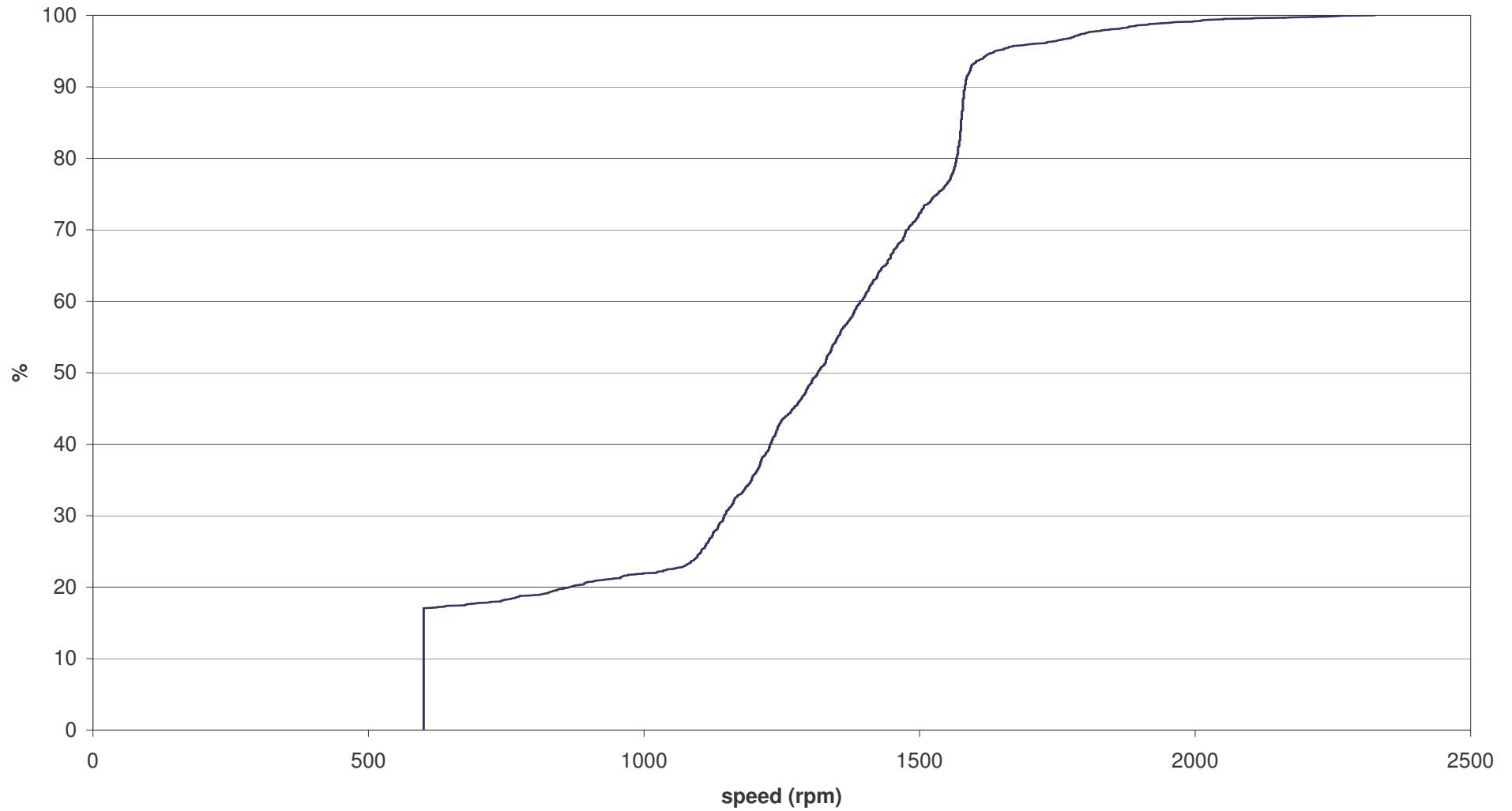
WHTC Speed vs Cumulative Frequency - Example 5 litre engine
