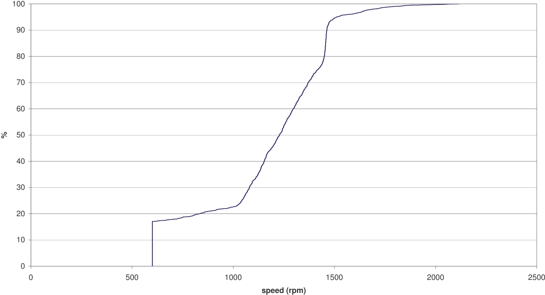
WHTC Speed vs Cumulative Frequency - Example 7 litre engine
