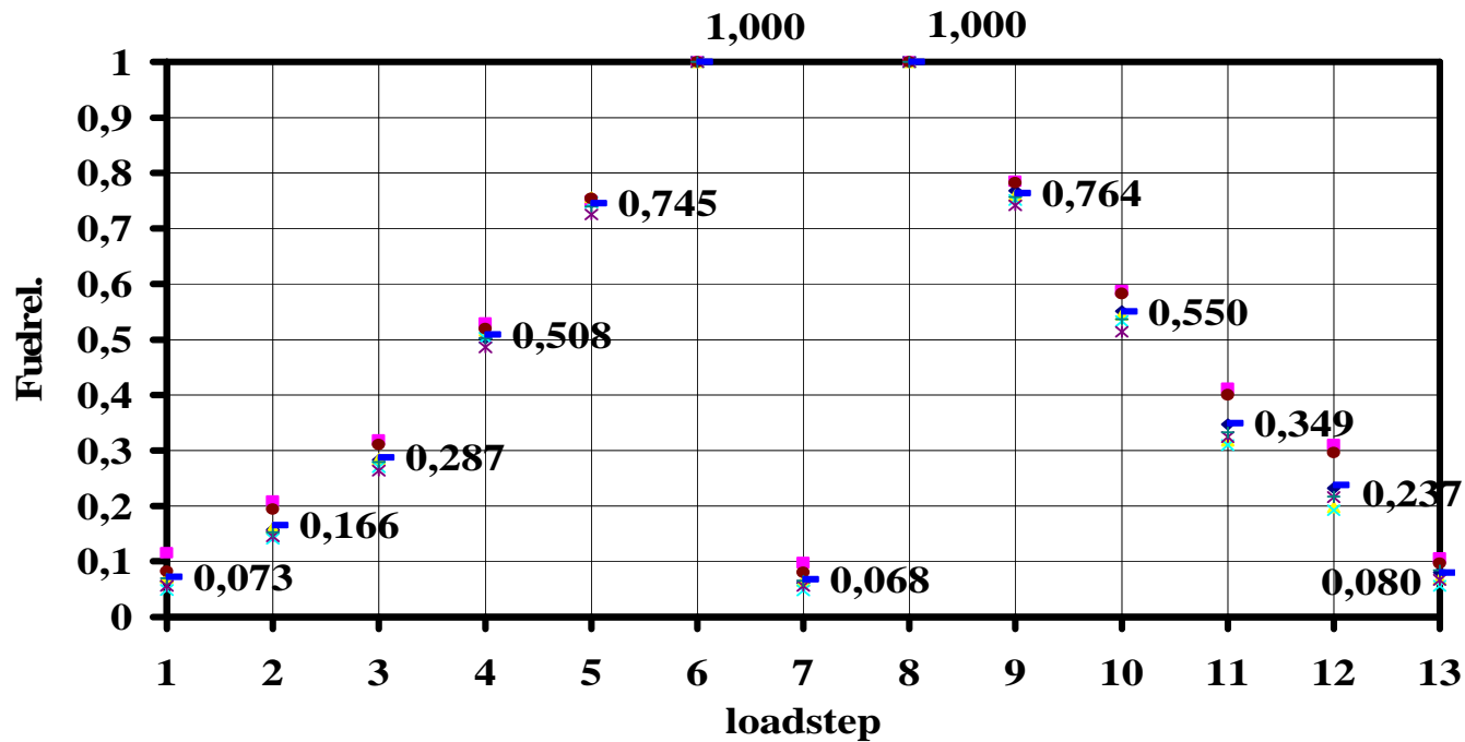
Relationship of fuelconsumption at 13 stepmode test
