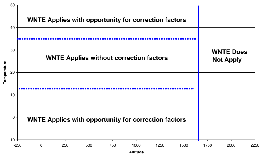
WNTe Altitude and Temperature Range: Option A
