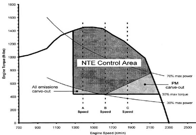
Figure 1. Example Not-To-Exceed Control Area When C Speed < 2,400 rpm
